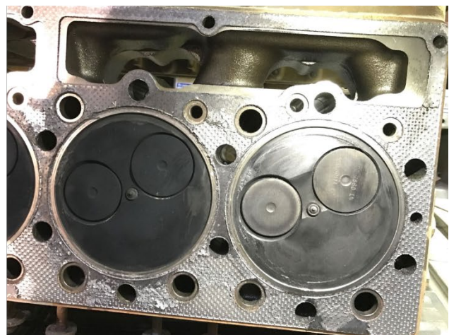
CAT 972G Loader Engine Disarmed, 10,000 hrs maintenance (3,000 hrs using FEROX by RENNSLI)
